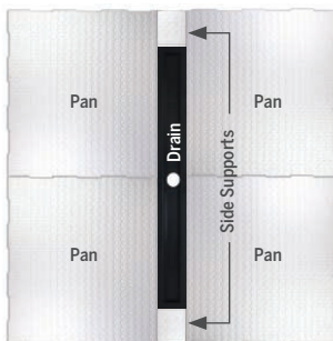
CENTER DRAIN - 4' X 4' (122 cm x 122 cm)
