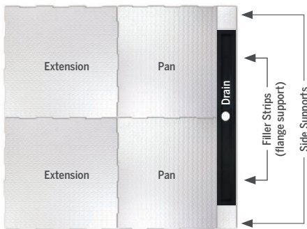
CENTER DRAIN - 4' X 4' (122 cm x 122 cm)
